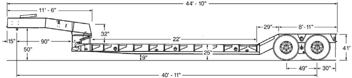
TANDEM AXLE MODEL SHOWN
